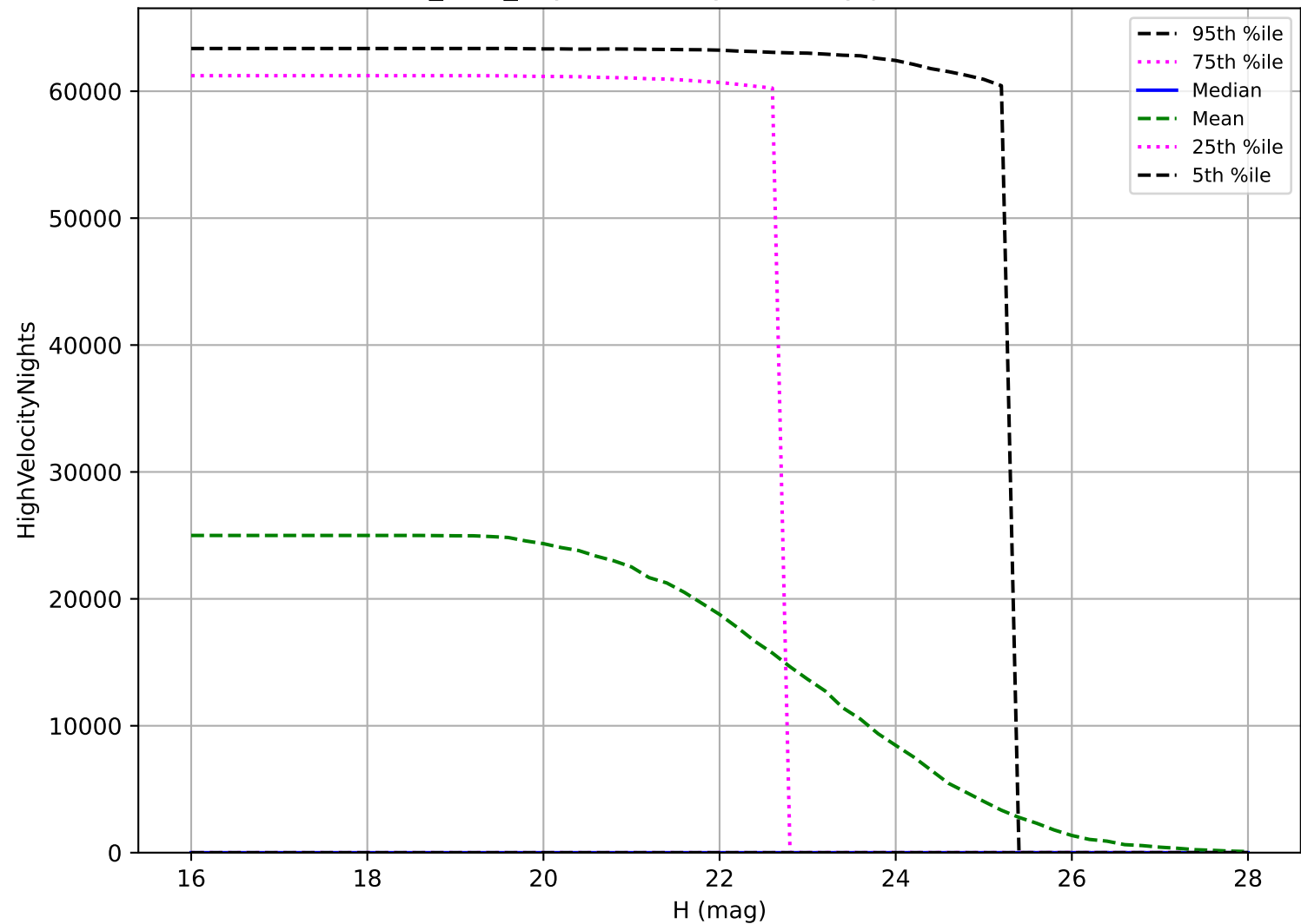
baseline_v2.0_10yrs: PHA High velocity pair detection loss
