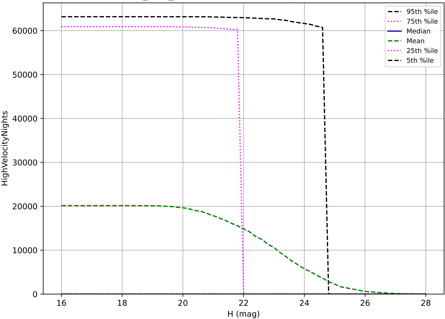
baseline_v2.0_10yrs: NEO High velocity pair detection loss
