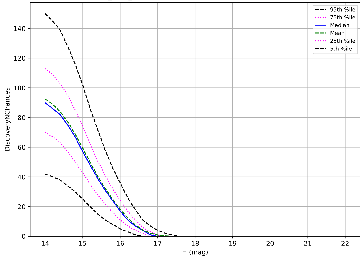
baseline_v2.0_10yrs: Trojan 3 pairs in 15 nights detection loss
