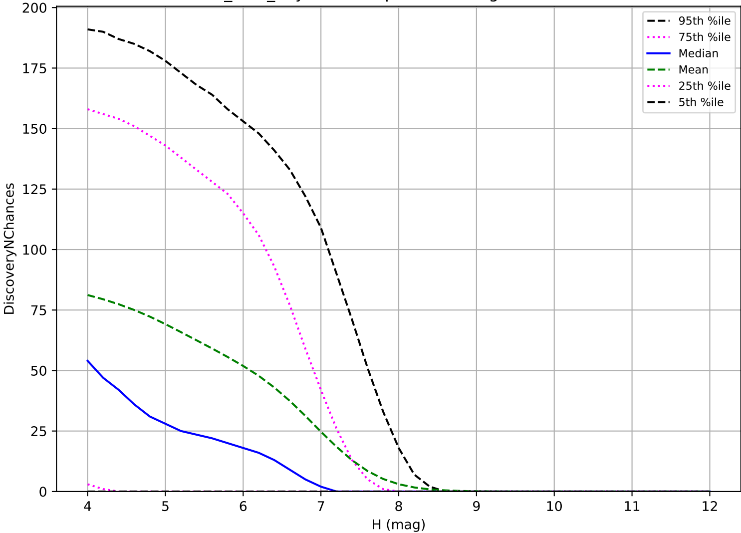
baseline_v2.0_10yrs: TNO 3 pairs in 15 nights detection loss
