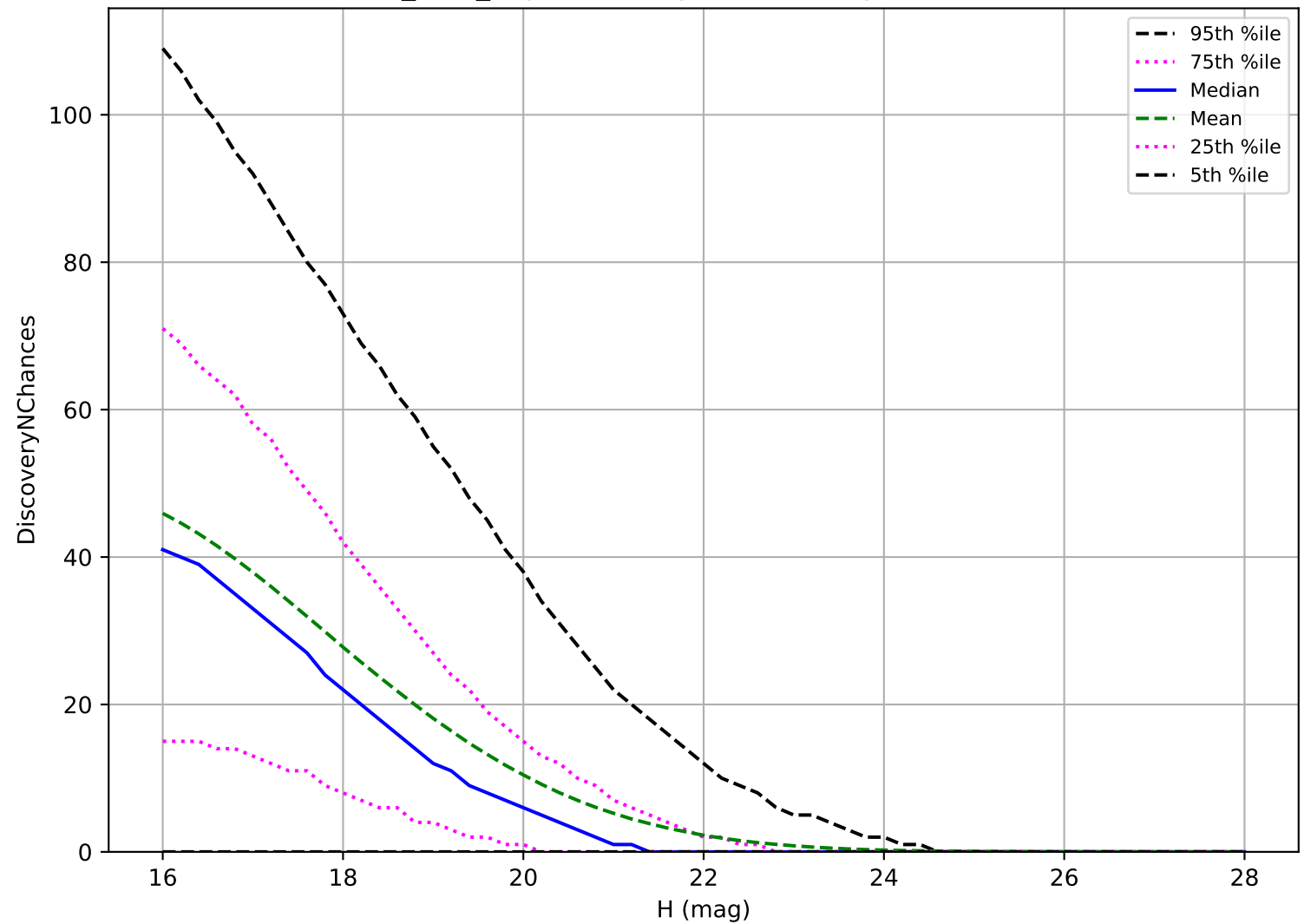
baseline_v2.0_10yrs: PHA 3 pairs in 15 nights detection loss
