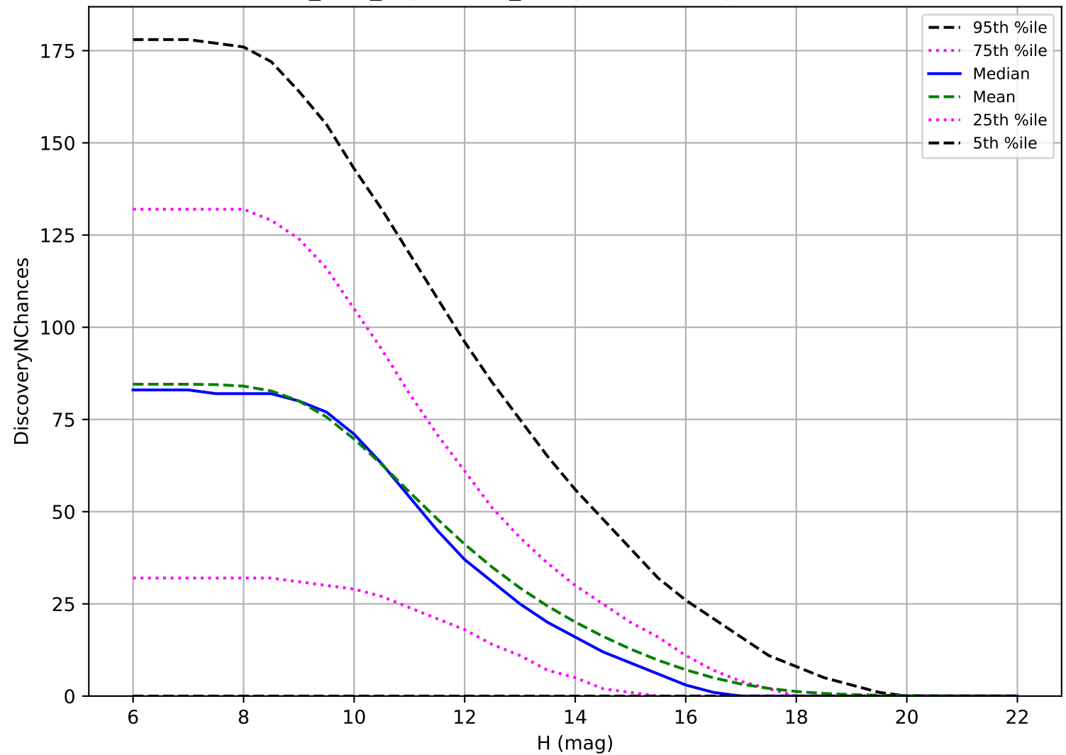
baseline_v2.0_10yrs: OCC_r5 3 pairs in 15 nights detection loss
