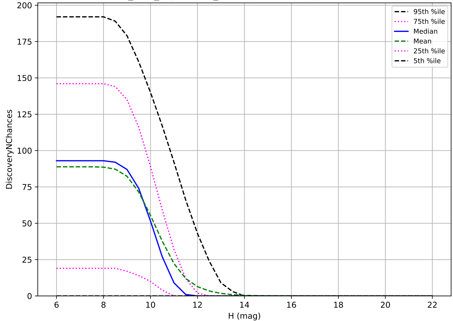
baseline_v2.0_10yrs: OCC_r20 3 pairs in 15 nights detection loss
