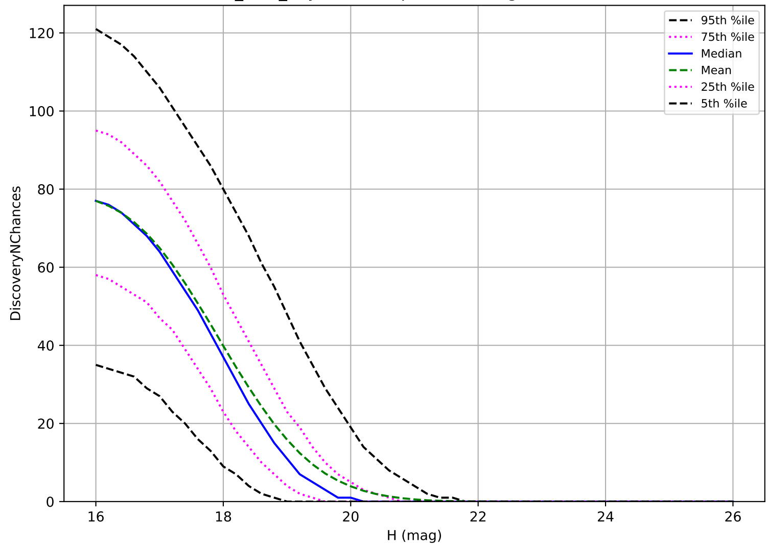
baseline_v2.0_10yrs: MBA 3 pairs in 15 nights detection loss
