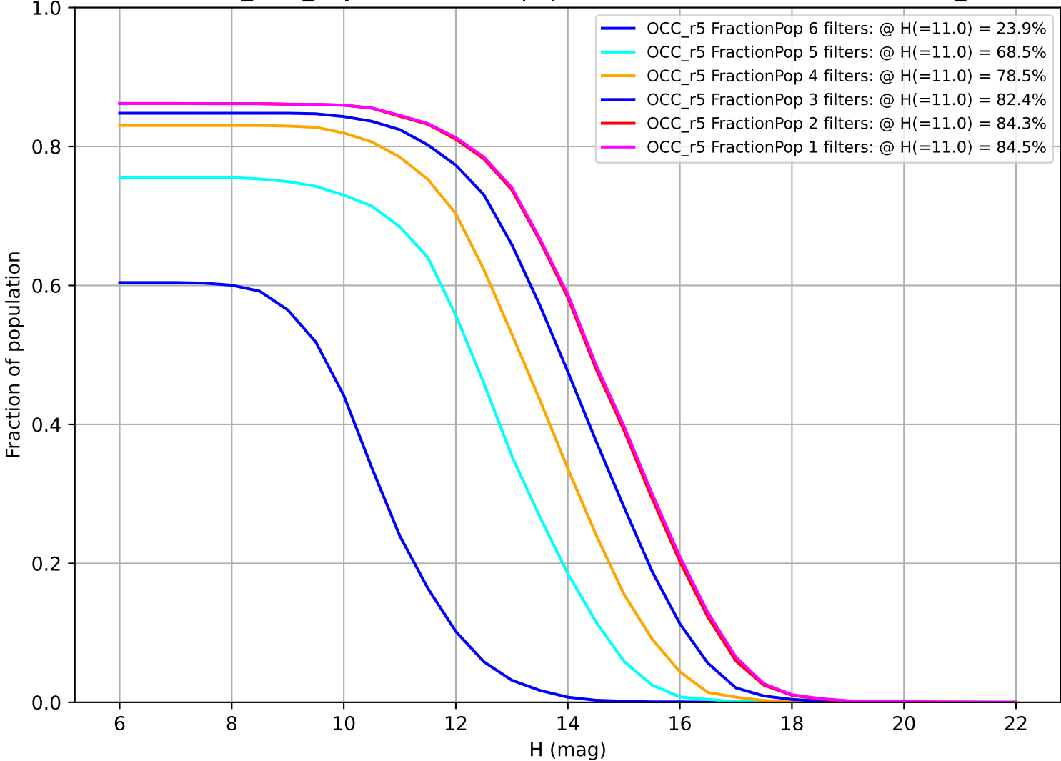
baseline_v2.0_10yrs: Fraction of population with colors in X filters OCC_r5
