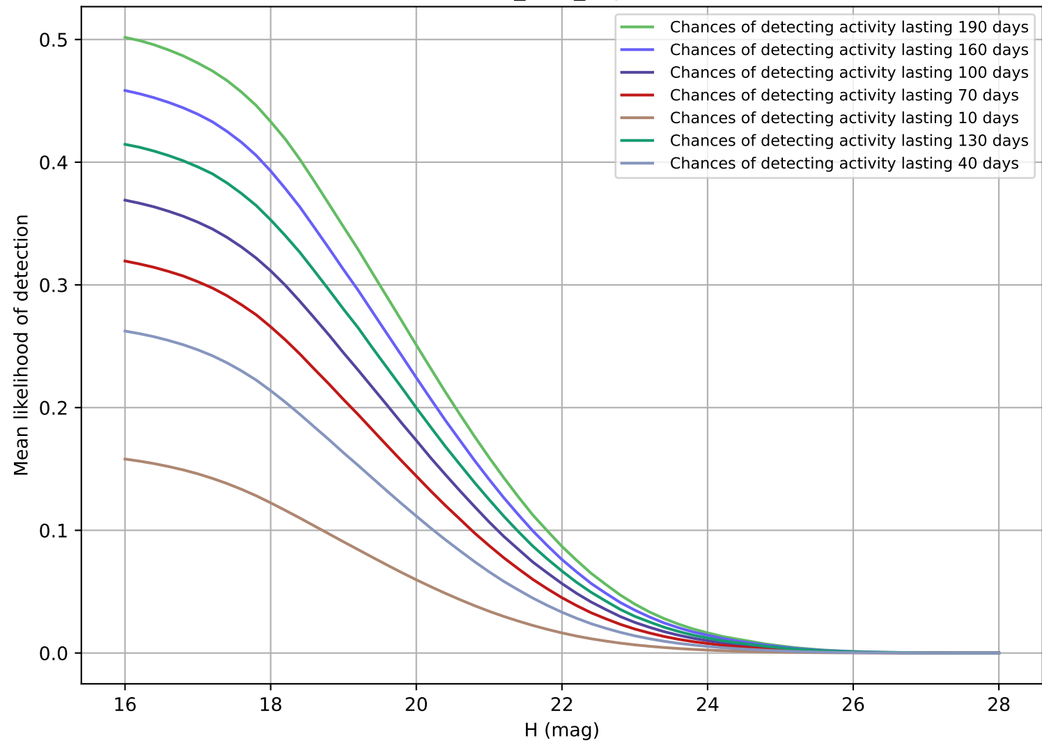
baseline_v2.0_10yrs NEO
