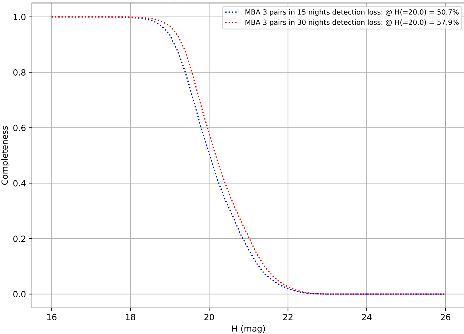
baseline_v2.0_10yrs: DifferentialCompleteness
