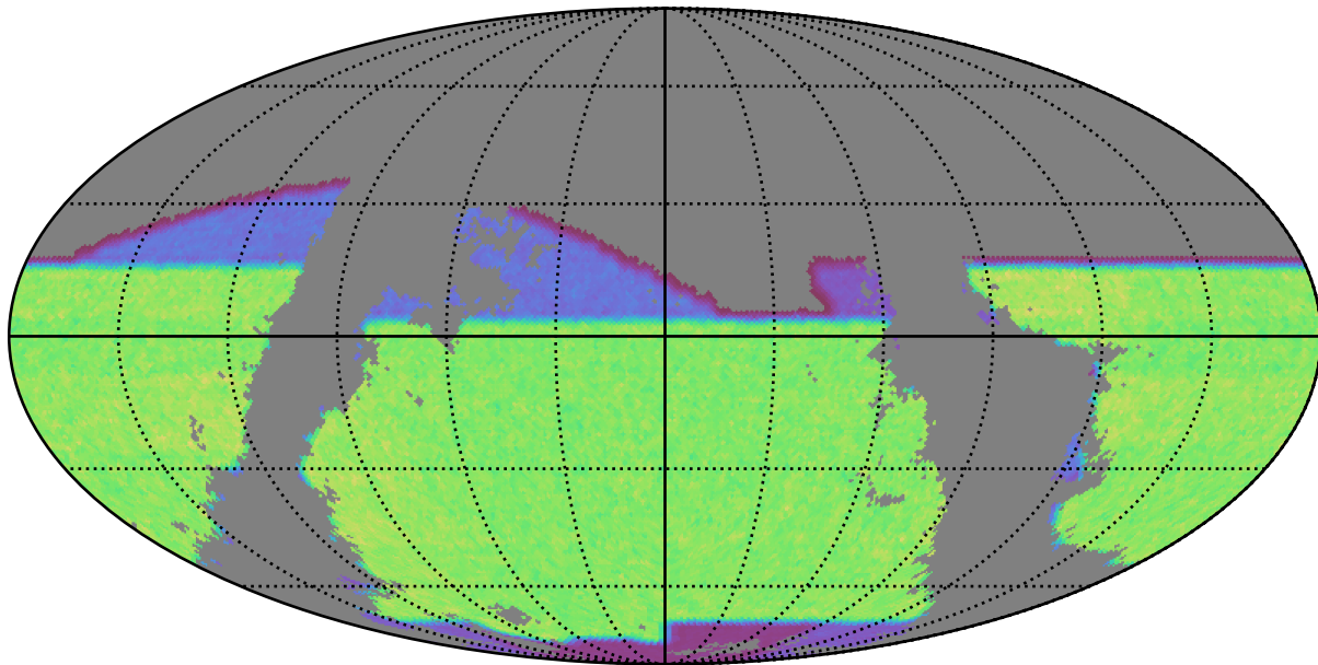
baseline_v2.0_10yrs gri band non-DD: riz_exposure_time_year8
