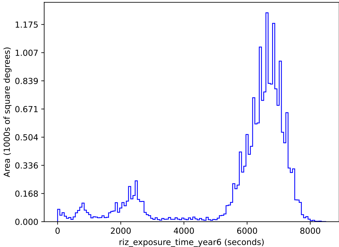
baseline_v2.0_10yrs gri band non-DD: riz_exposure_time_year6
