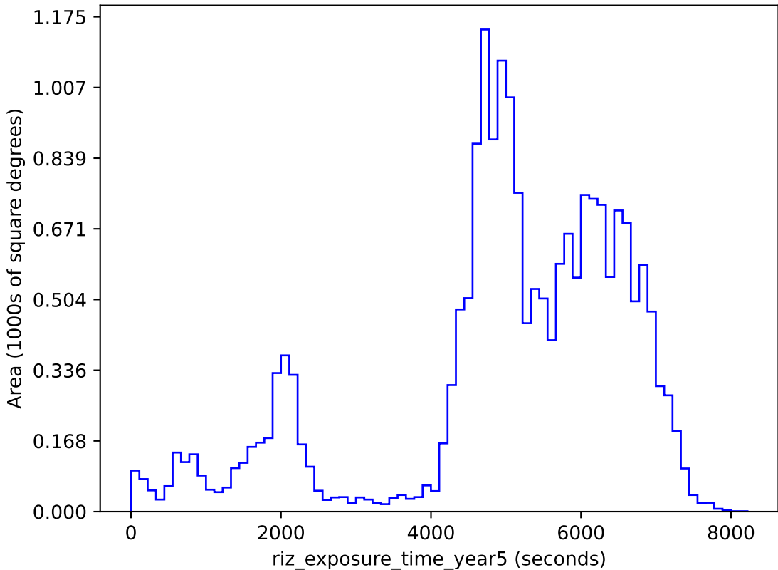
baseline_v2.0_10yrs gri band non-DD: riz_exposure_time_year5
