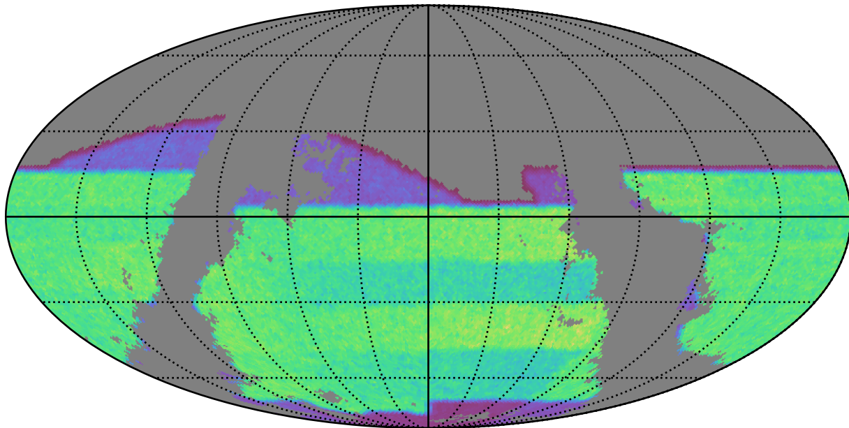
baseline_v2.0_10yrs gri band non-DD: riz_exposure_time_year4
