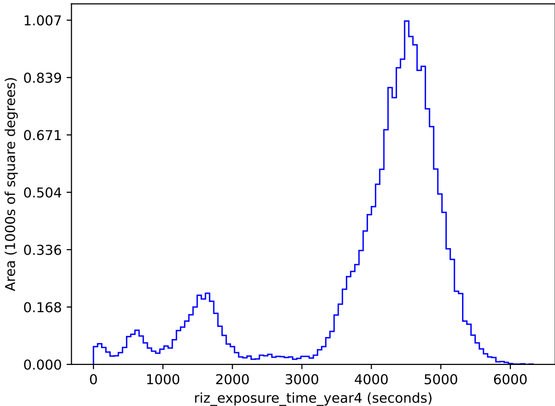
baseline_v2.0_10yrs gri band non-DD: riz_exposure_time_year4
