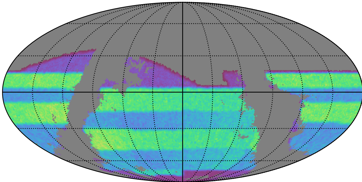
baseline_v2.0_10yrs gri band non-DD: riz_exposure_time_year3
