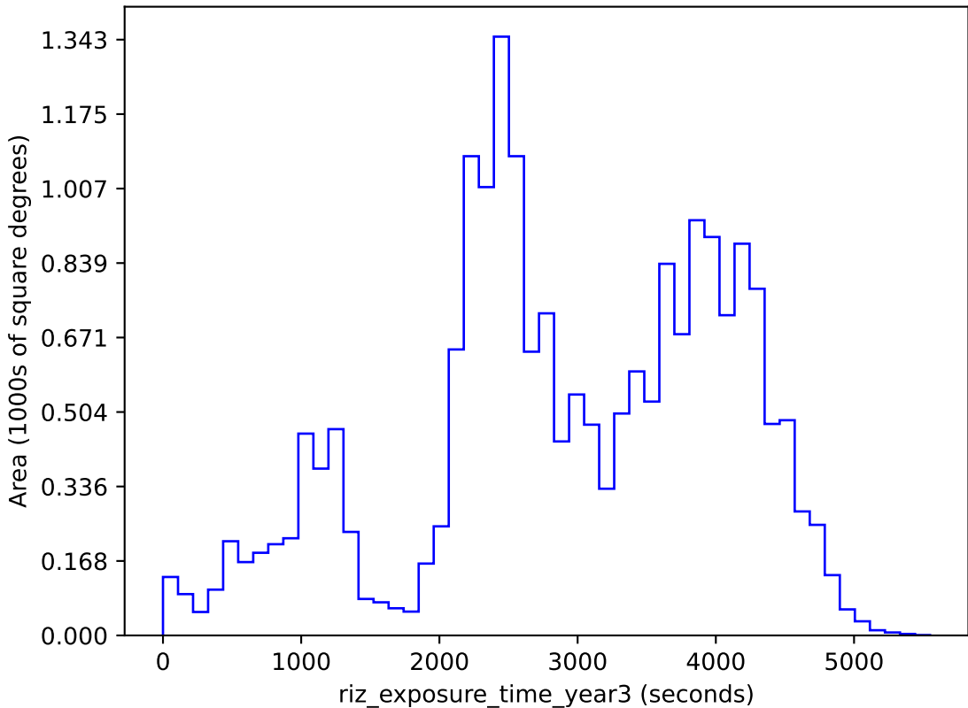
baseline_v2.0_10yrs gri band non-DD: riz_exposure_time_year3
