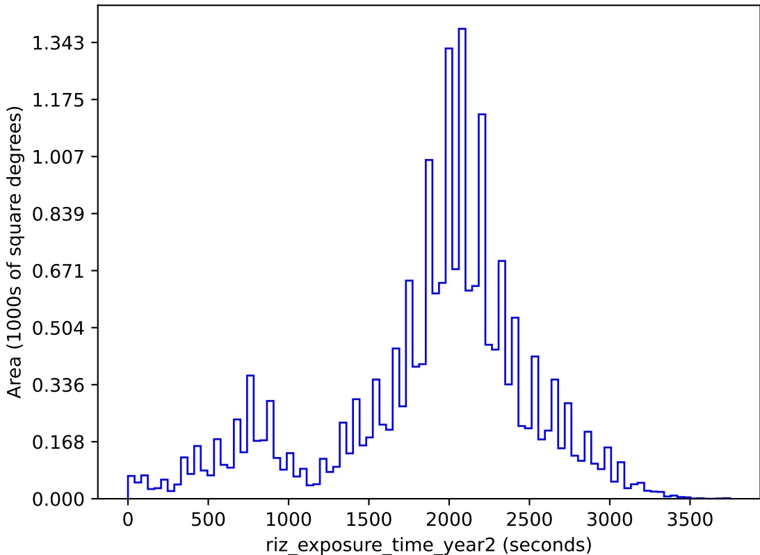
baseline_v2.0_10yrs gri band non-DD: riz_exposure_time_year2
