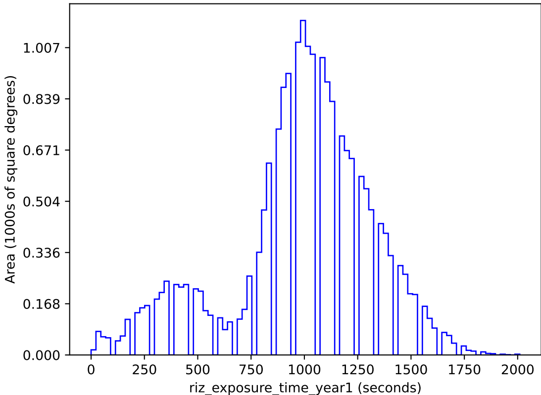
baseline_v2.0_10yrs gri band non-DD: riz_exposure_time_year1
