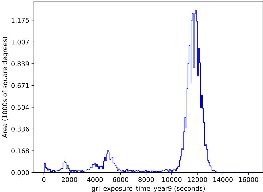
baseline_v2.0_10yrs gri band non-DD: gri_exposure_time_year9
