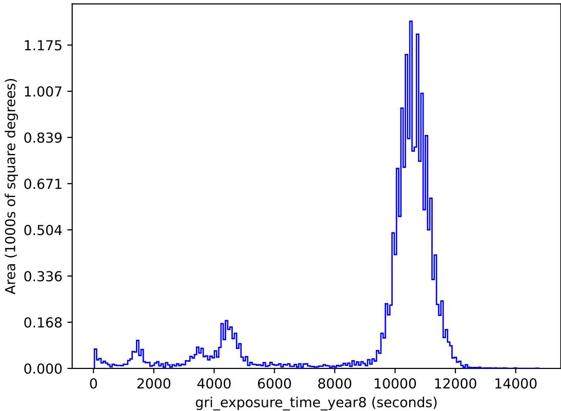
baseline_v2.0_10yrs gri band non-DD: gri_exposure_time_year8
