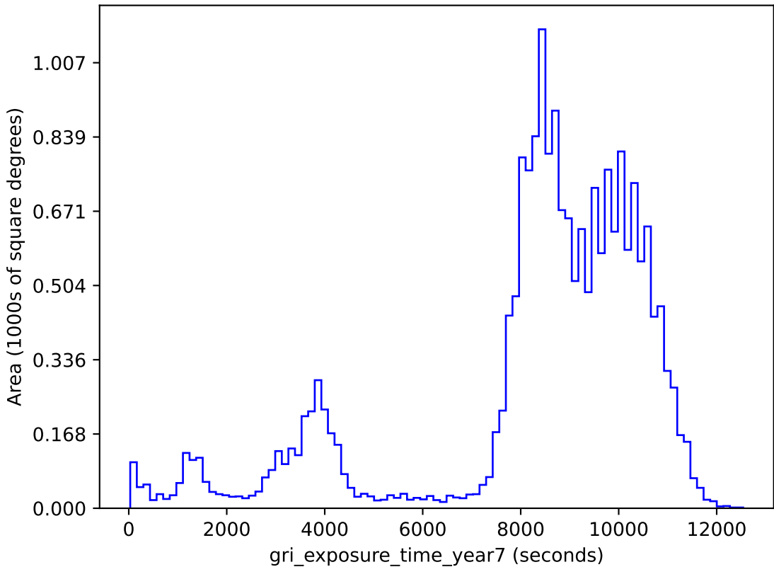
baseline_v2.0_10yrs gri band non-DD: gri_exposure_time_year7
