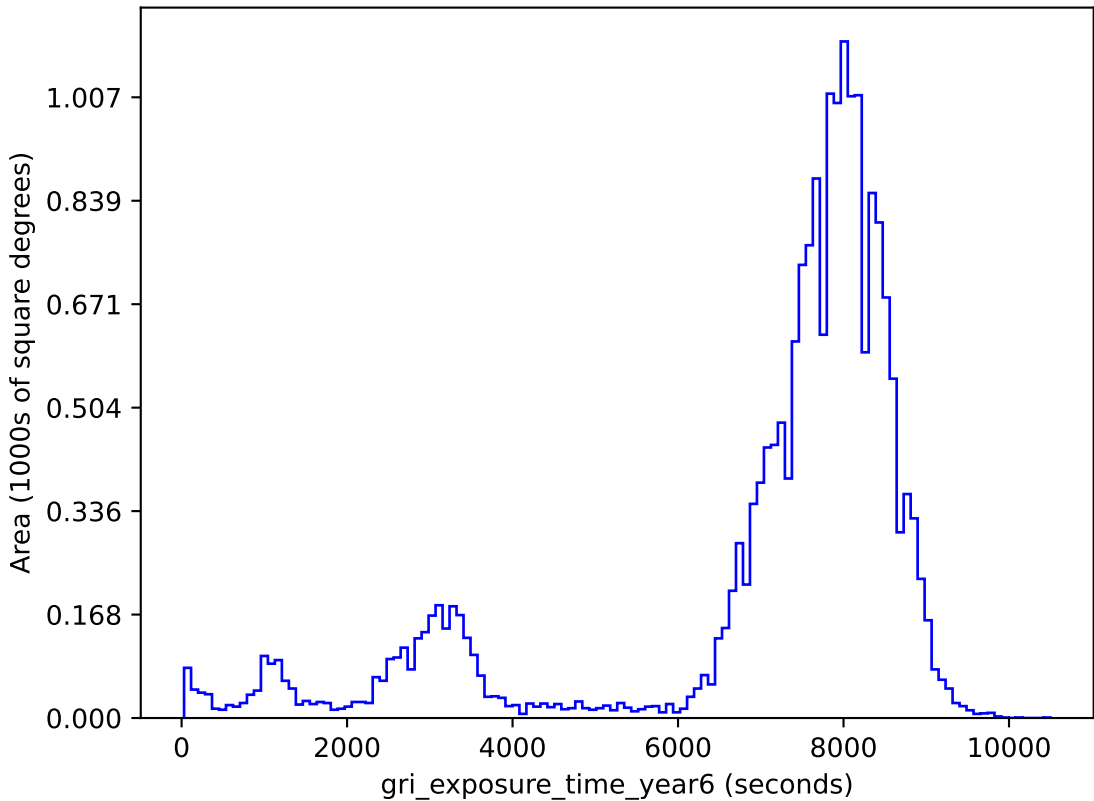
baseline_v2.0_10yrs gri band non-DD: gri_exposure_time_year6
