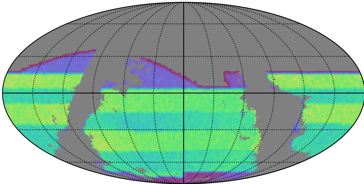
baseline_v2.0_10yrs gri band non-DD: gri_exposure_time_year5
