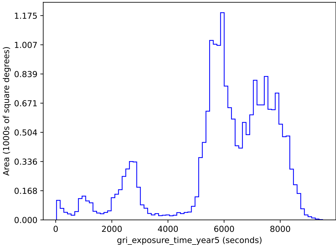
baseline_v2.0_10yrs gri band non-DD: gri_exposure_time_year5
