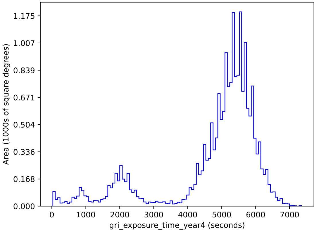
baseline_v2.0_10yrs gri band non-DD: gri_exposure_time_year4
