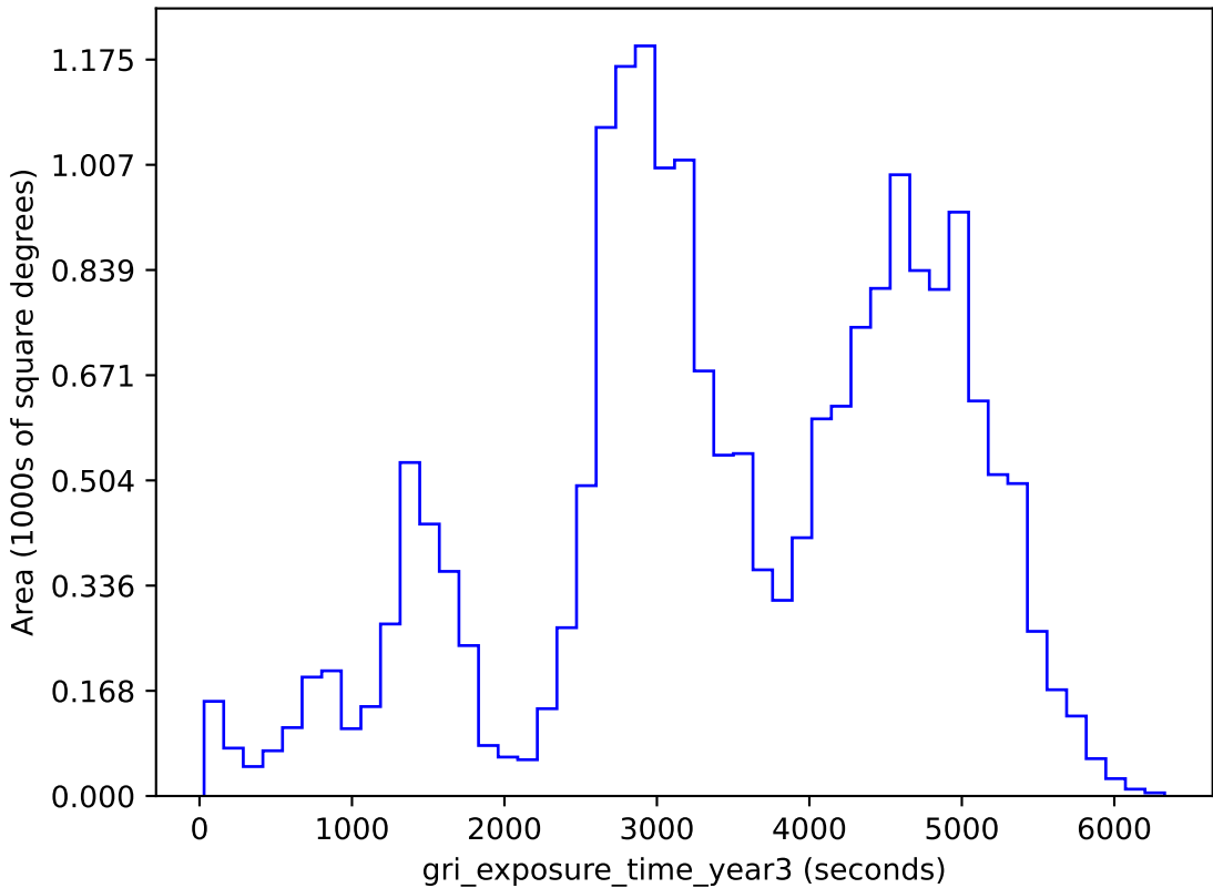
baseline_v2.0_10yrs gri band non-DD: gri_exposure_time_year3
