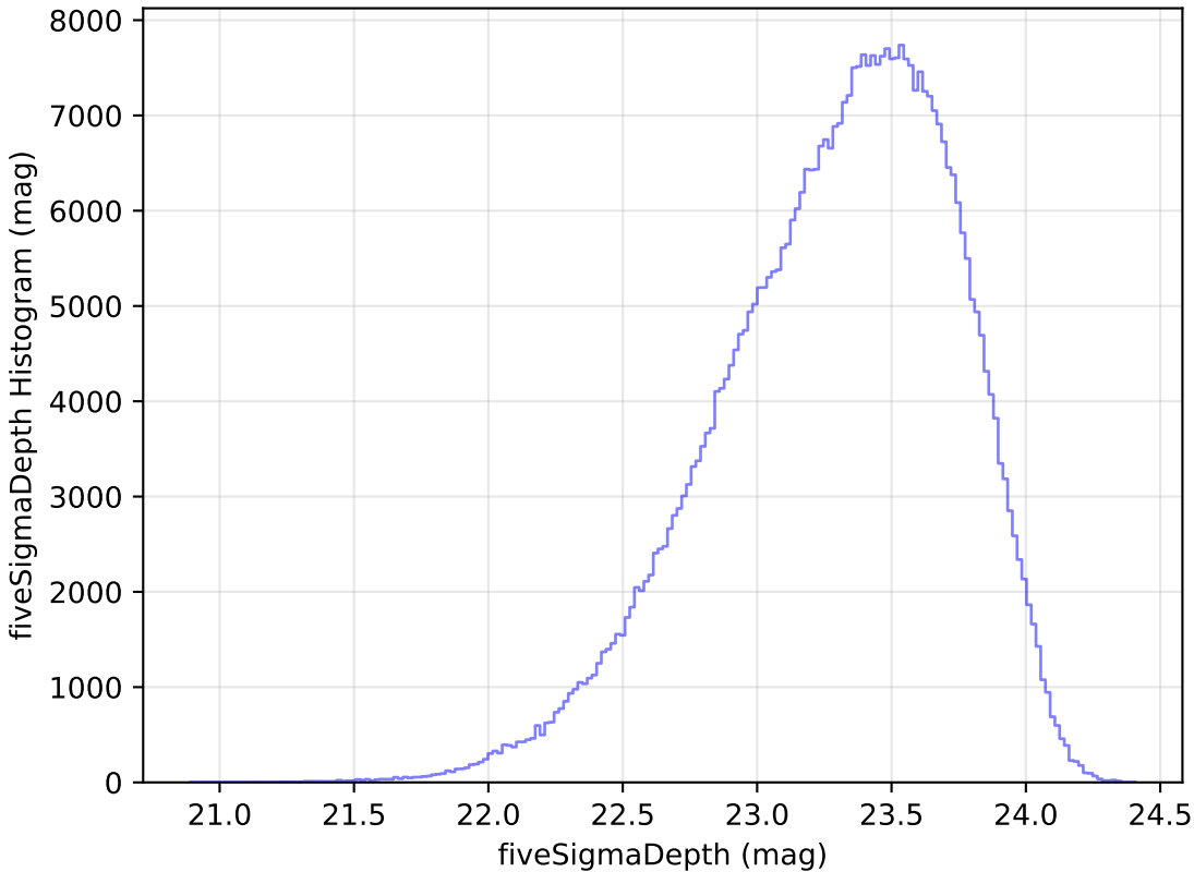
baseline_v2.0_10yrs i: fiveSigmaDepth Histogram
