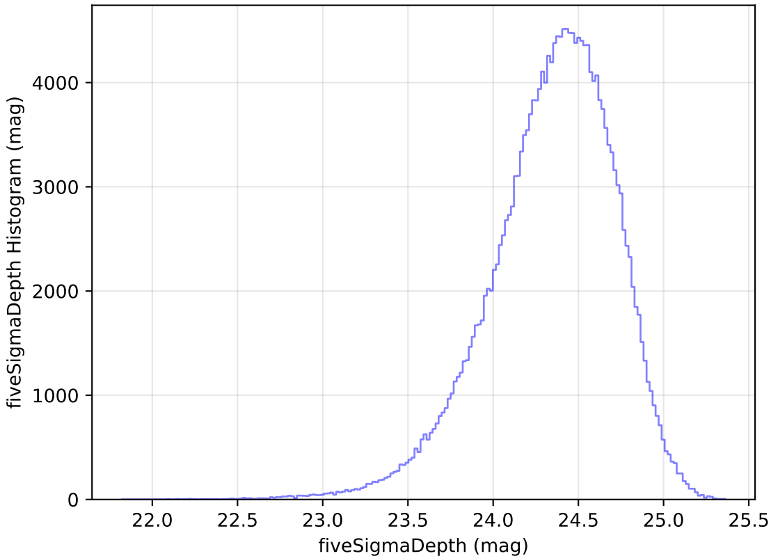
baseline_v2.0_10yrs g: fiveSigmaDepth Histogram
