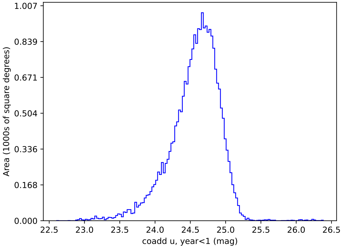
baseline_v2.0_10yrs night<365 and u: coadd u, year<1
