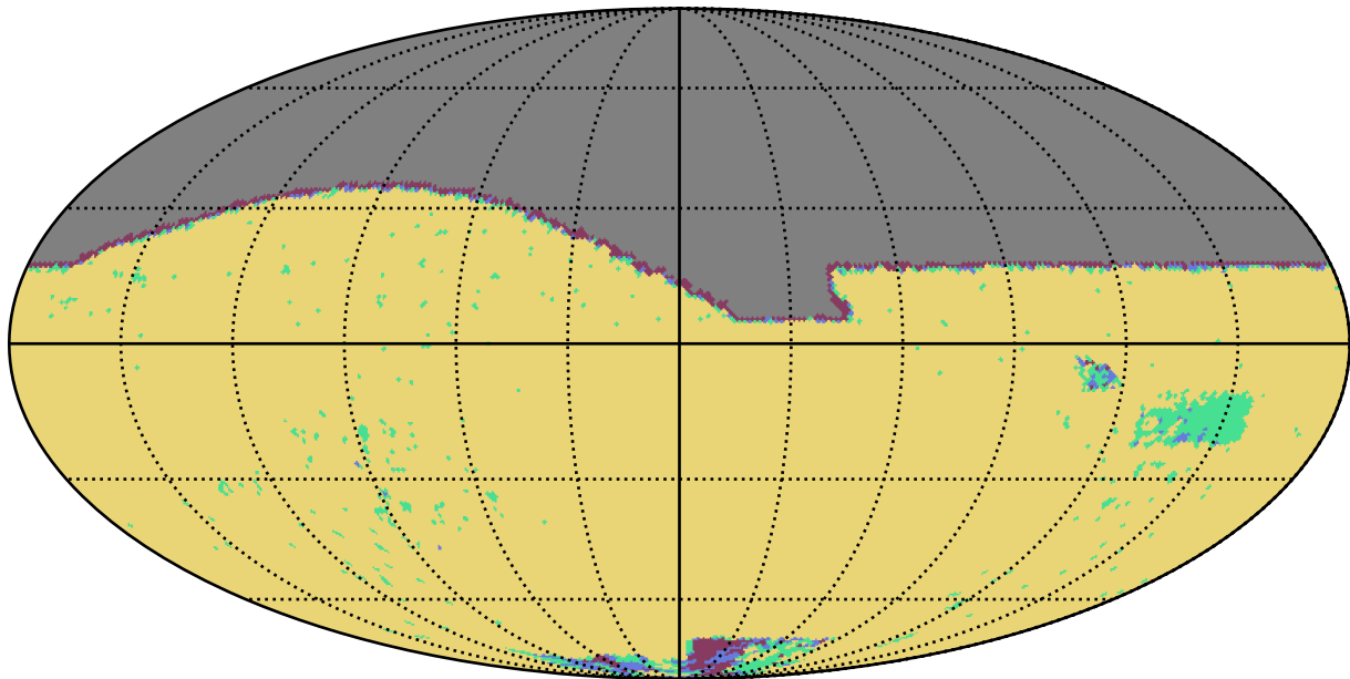
baseline_v2.0_10yrs z band: YearCoverage night
