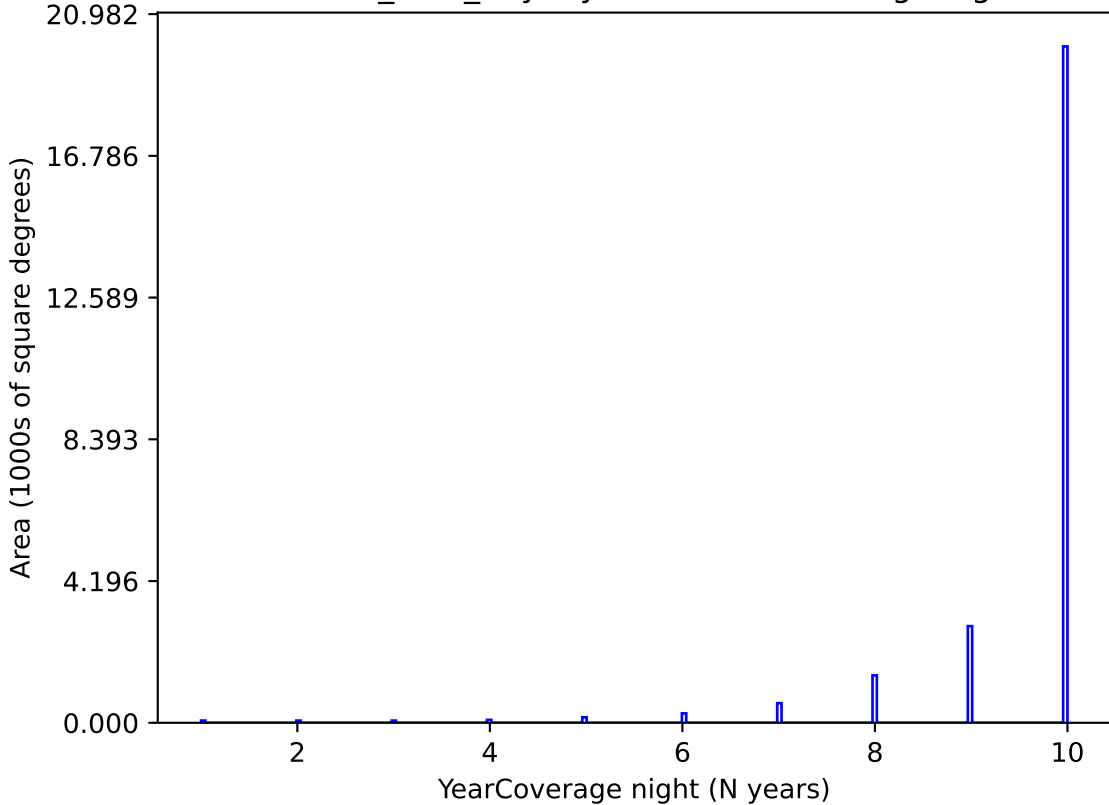
baseline_v2.0_10yrs y band: YearCoverage night
