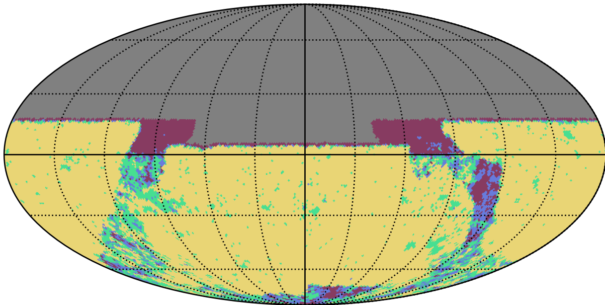
baseline_v2.0_10yrs u band: YearCoverage night
