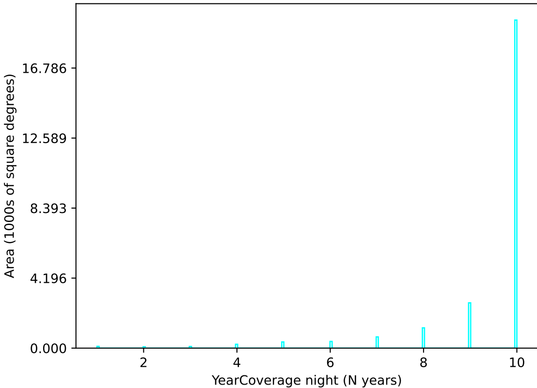
baseline_v2.0_10yrs u band: YearCoverage night
