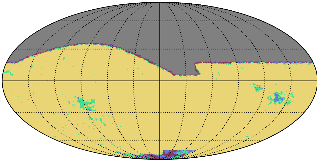
baseline_v2.0_10yrs r band: YearCoverage night
