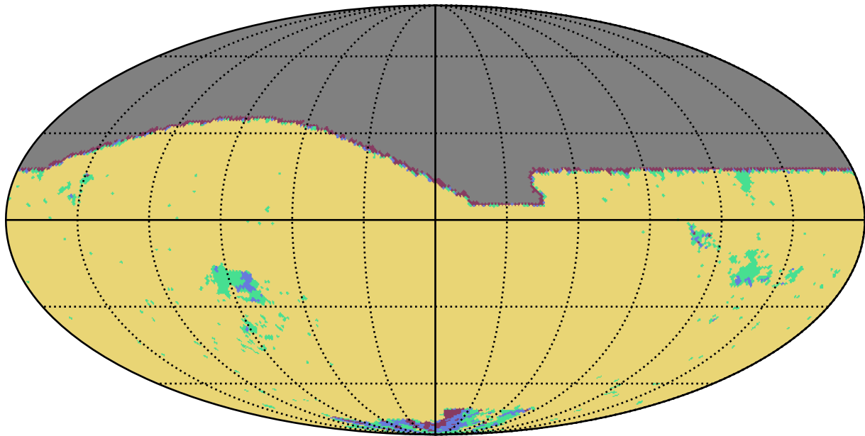
baseline_v2.0_10yrs i band: YearCoverage night
