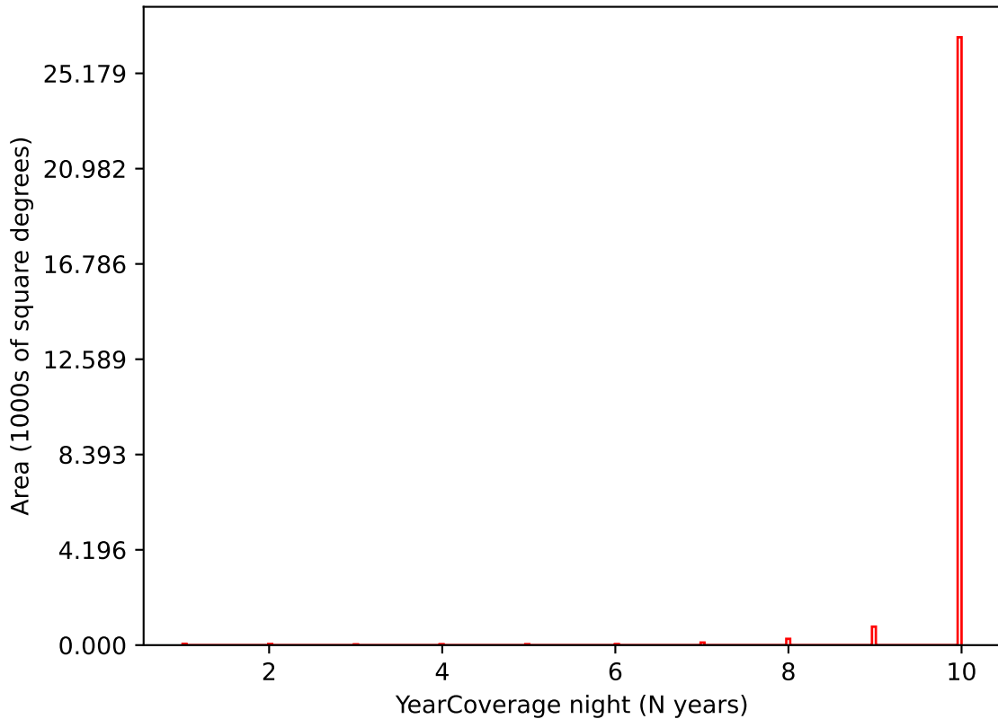
baseline_v2.0_10yrs i band: YearCoverage night
