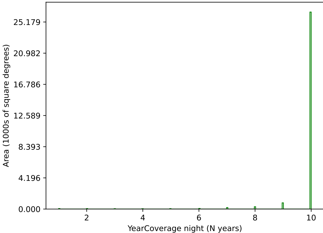
baseline_v2.0_10yrs g band: YearCoverage night
