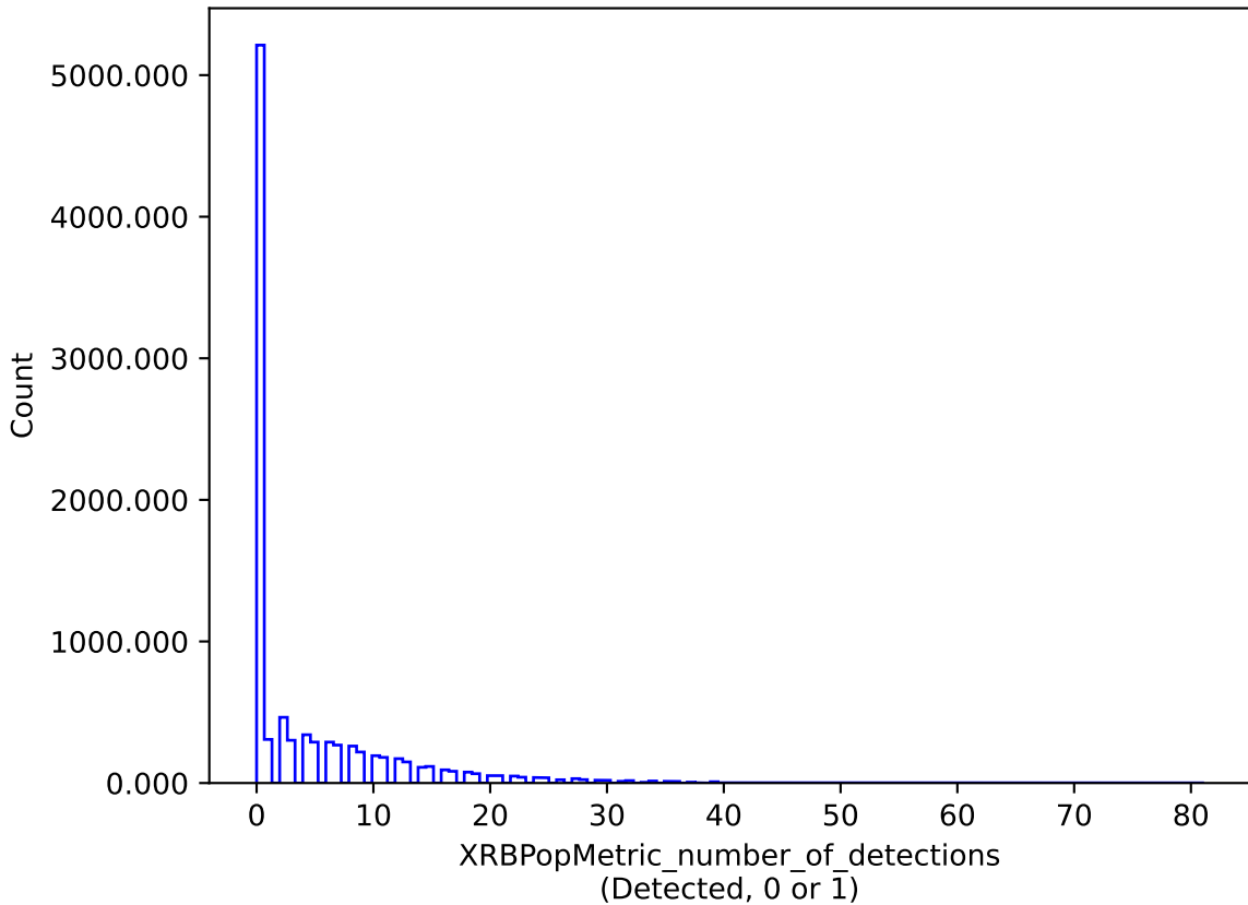
baseline_v2.0_10yrs : XRBPopMetric_number_of_detections
