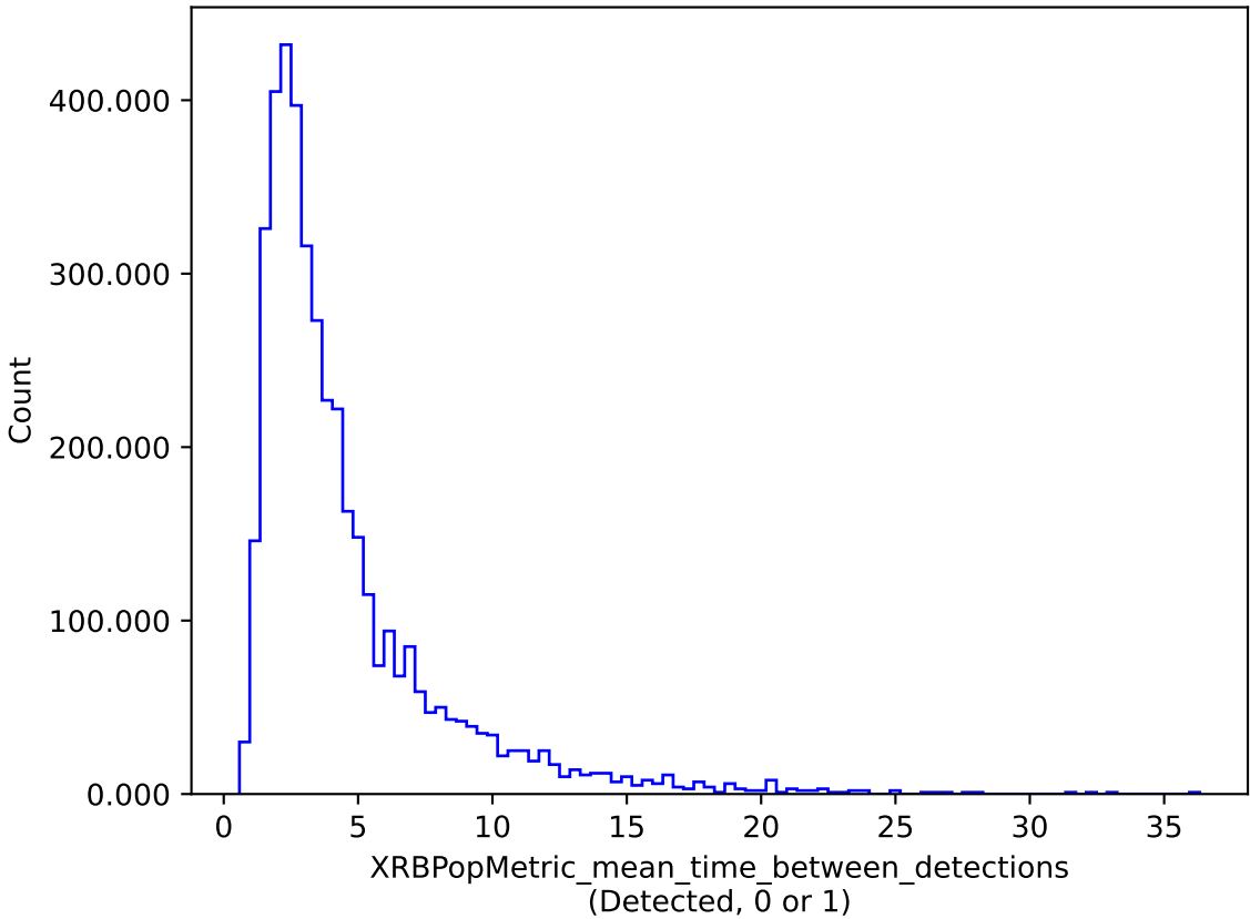
baseline_v2.0_10yrs : XRBPoMetric_mean_time_between_detections
