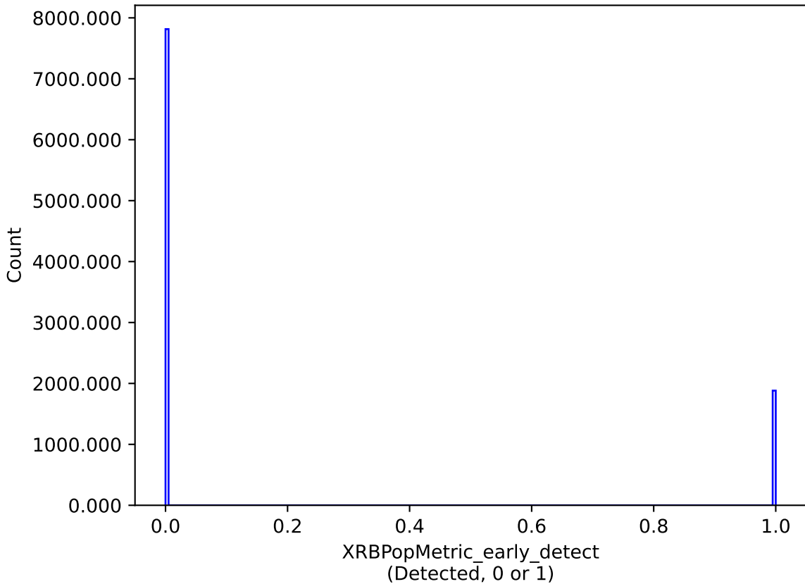
baseline_v2.0_10yrs : XRBPoMetric_early_detect
