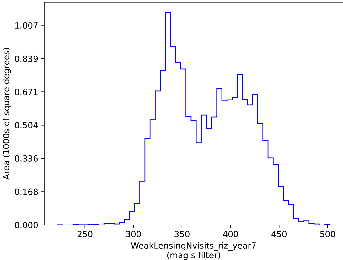
baseline_v2.0_10yrs gri band non-DD: WeakLensingNvisits_riz_year7
