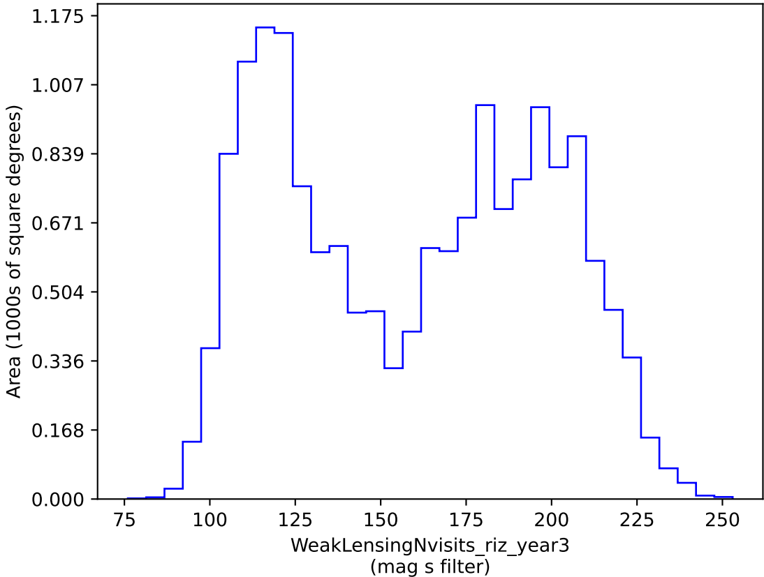
baseline_v2.0_10yrs gri band non-DD: WeakLensingNvisits_riz_year3
