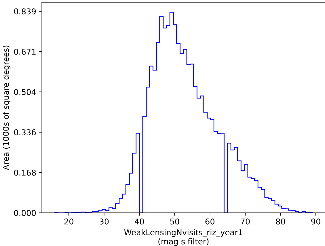
baseline_v2.0_10yrs gri band non-DD: WeakLensingNvisits_riz_year1
