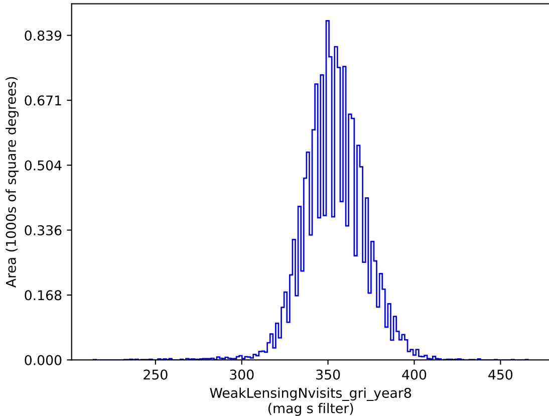
baseline_v2.0_10yrs gri band non-DD: WeakLensingNvisits_gri_year8
