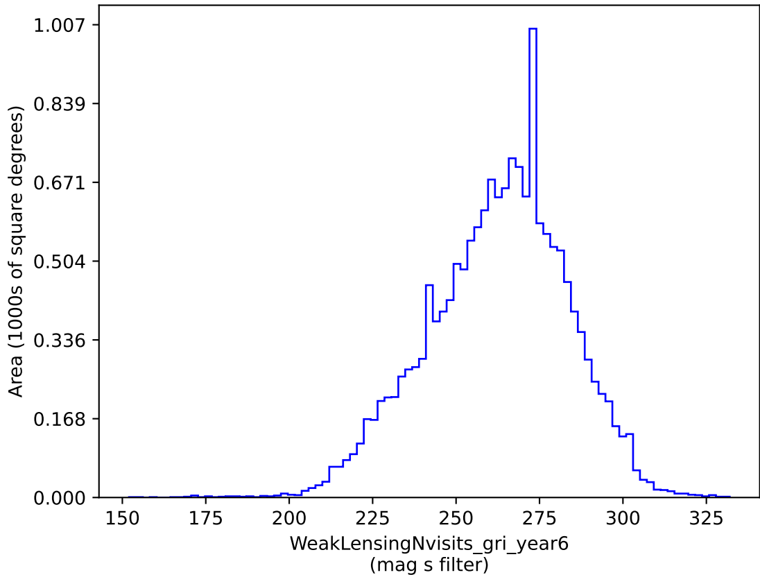
baseline_v2.0_10yrs gri band non-DD: WeakLensingNvisits_gri_year6
