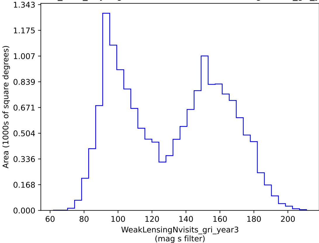
baseline_v2.0_10yrs gri band non-DD: WeakLensingNvisits_gri_year3
