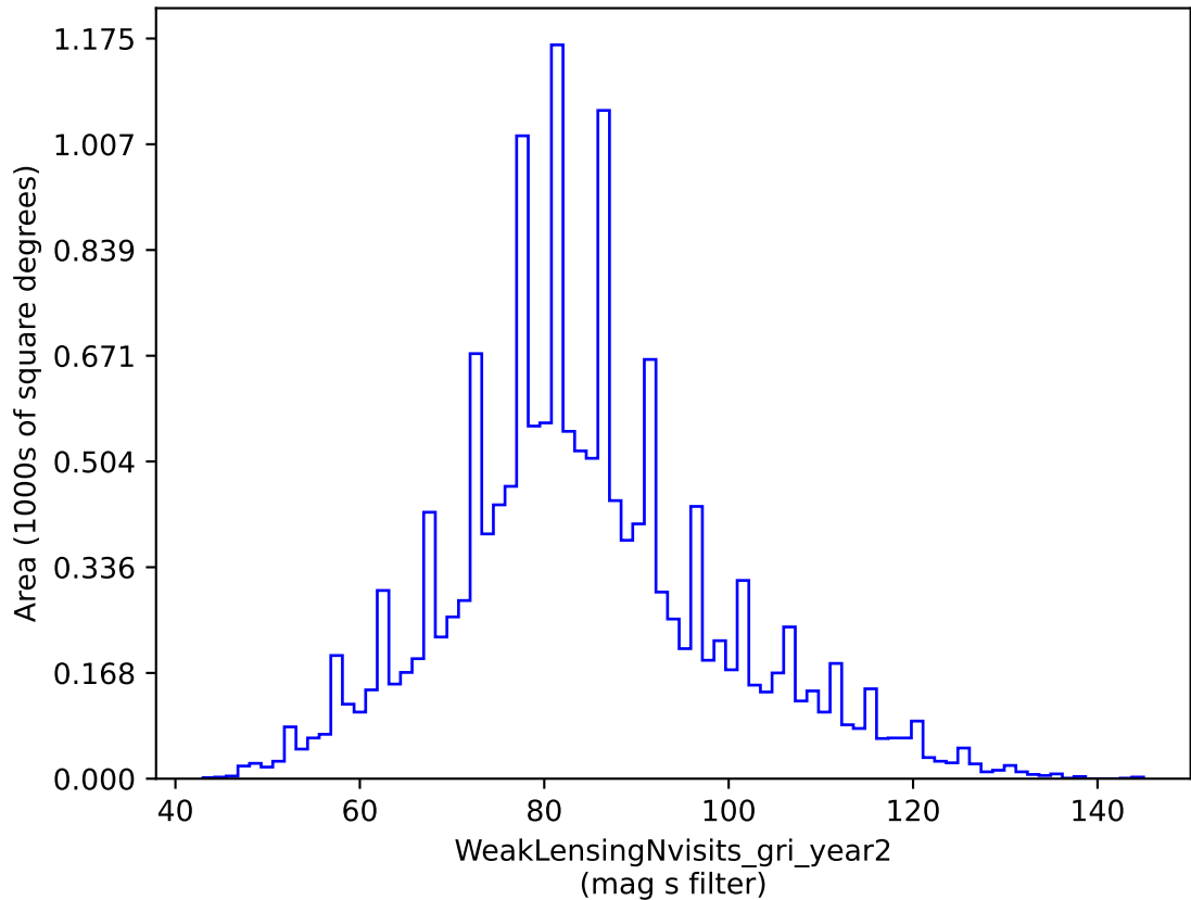
baseline_v2.0_10yrs gri band non-DD: WeakLensingNvisits_gri_year2
