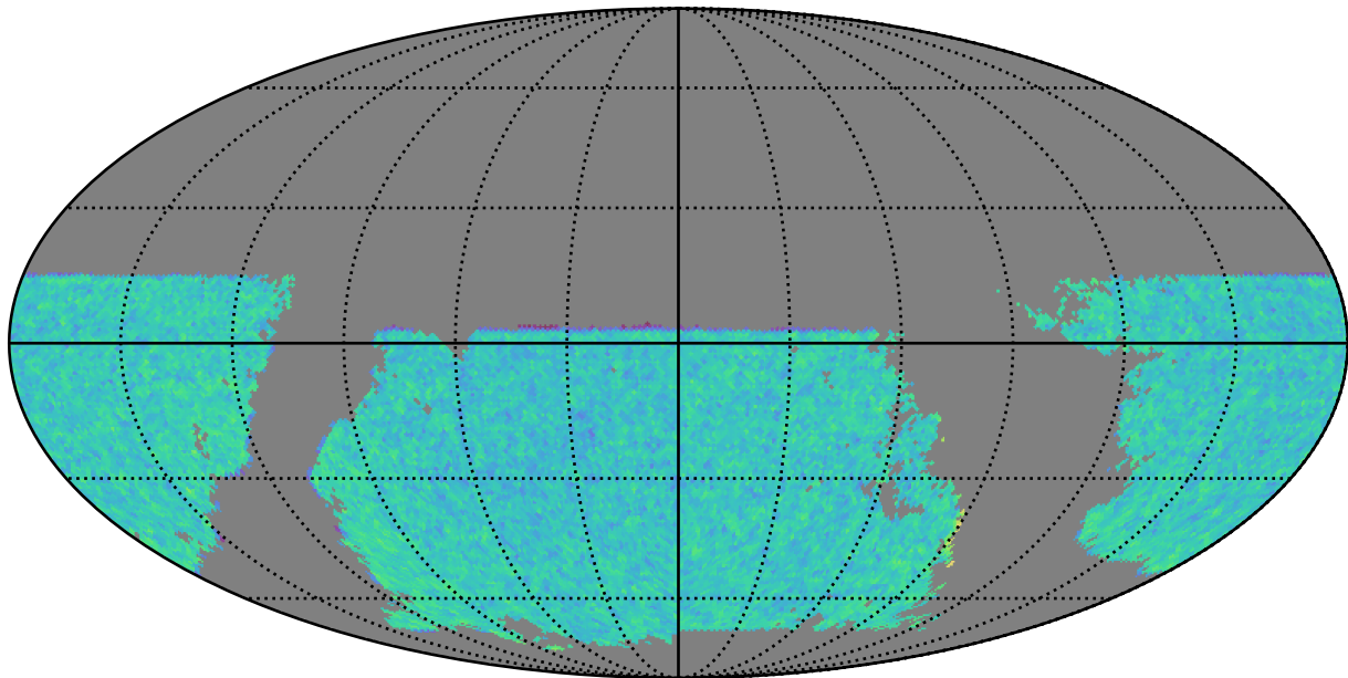
baseline_v2.0_10yrs gri band non-DD: WeakLensingNvisits
